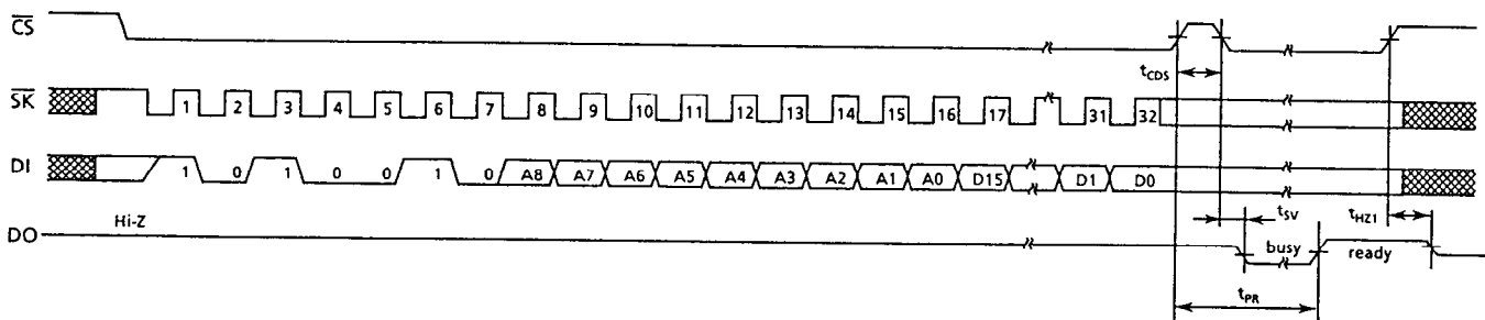
Figure 6 PROGRAM Timing
