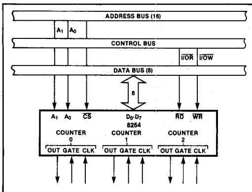
Figure 6. 8254 System Interface
