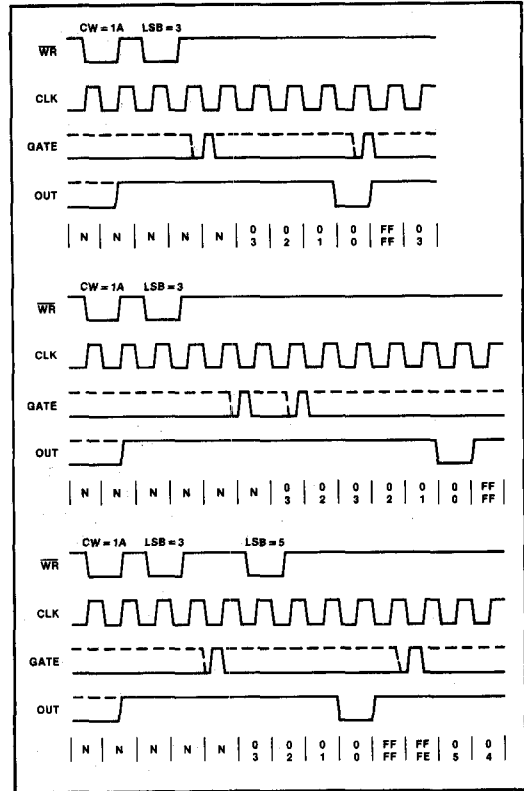
Figure 20. Mode 5
