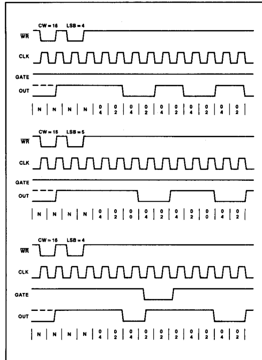
Figure 18. Mode 3
