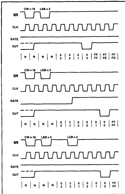
Figure 19. Mode 4
