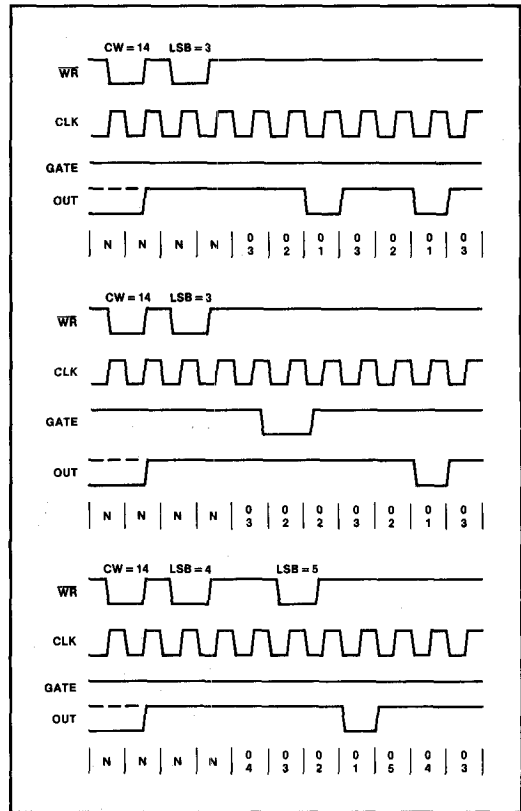
Figure 17. Mode 2
