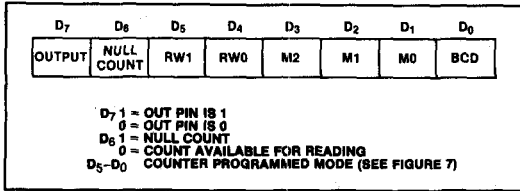
Figure 11. Status Byte
