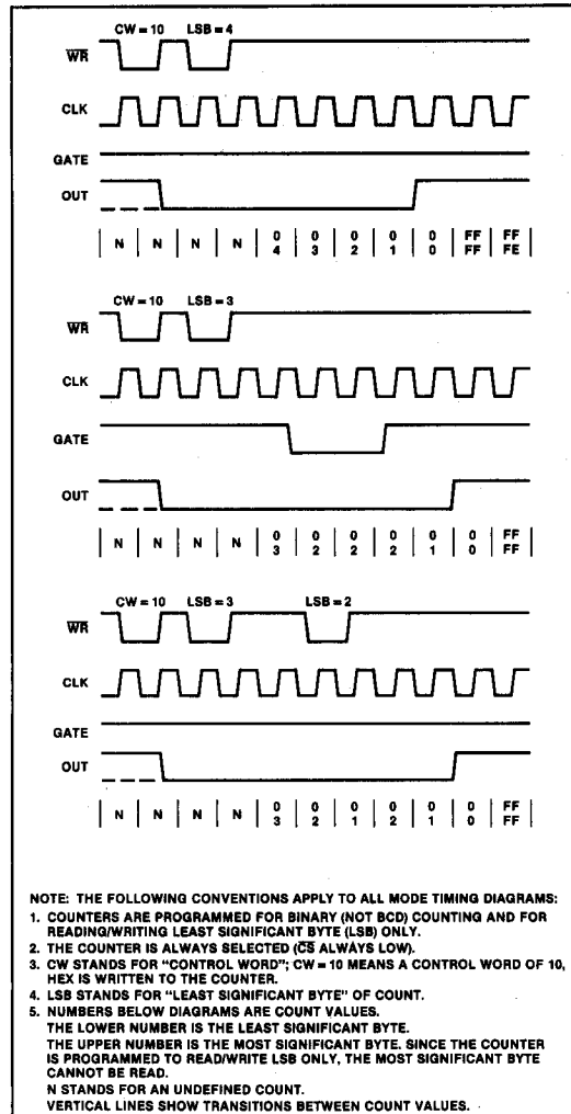
Figure 15. Mode 0
