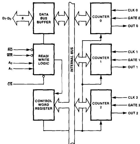
Figure 1. 8254 Block Diagram
