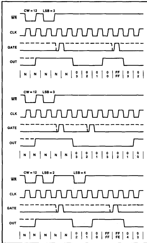
Figure 16. Mode 1
