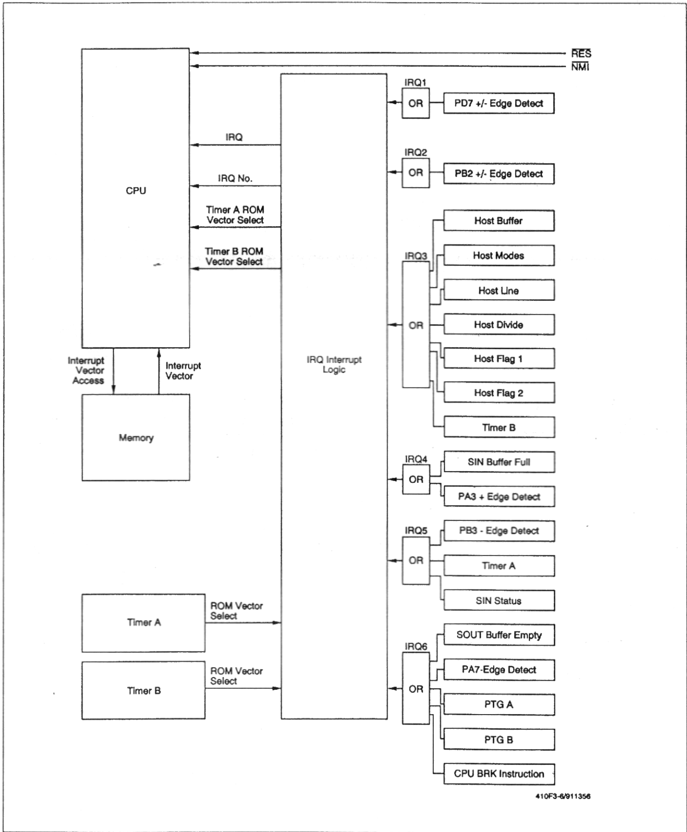
Figure 3-6. IRQ Interrupt Logic Interface
