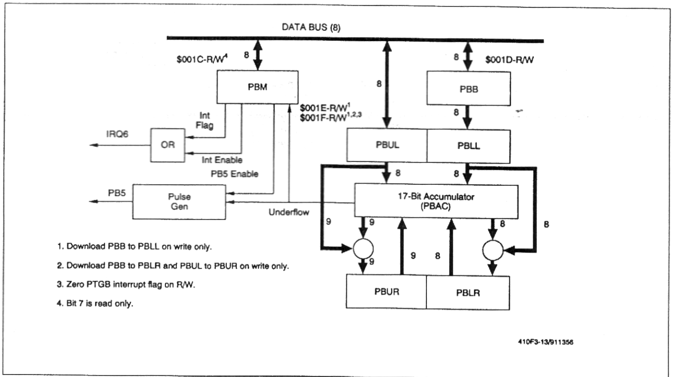
Figure 3-13. Precision Time Generator B
