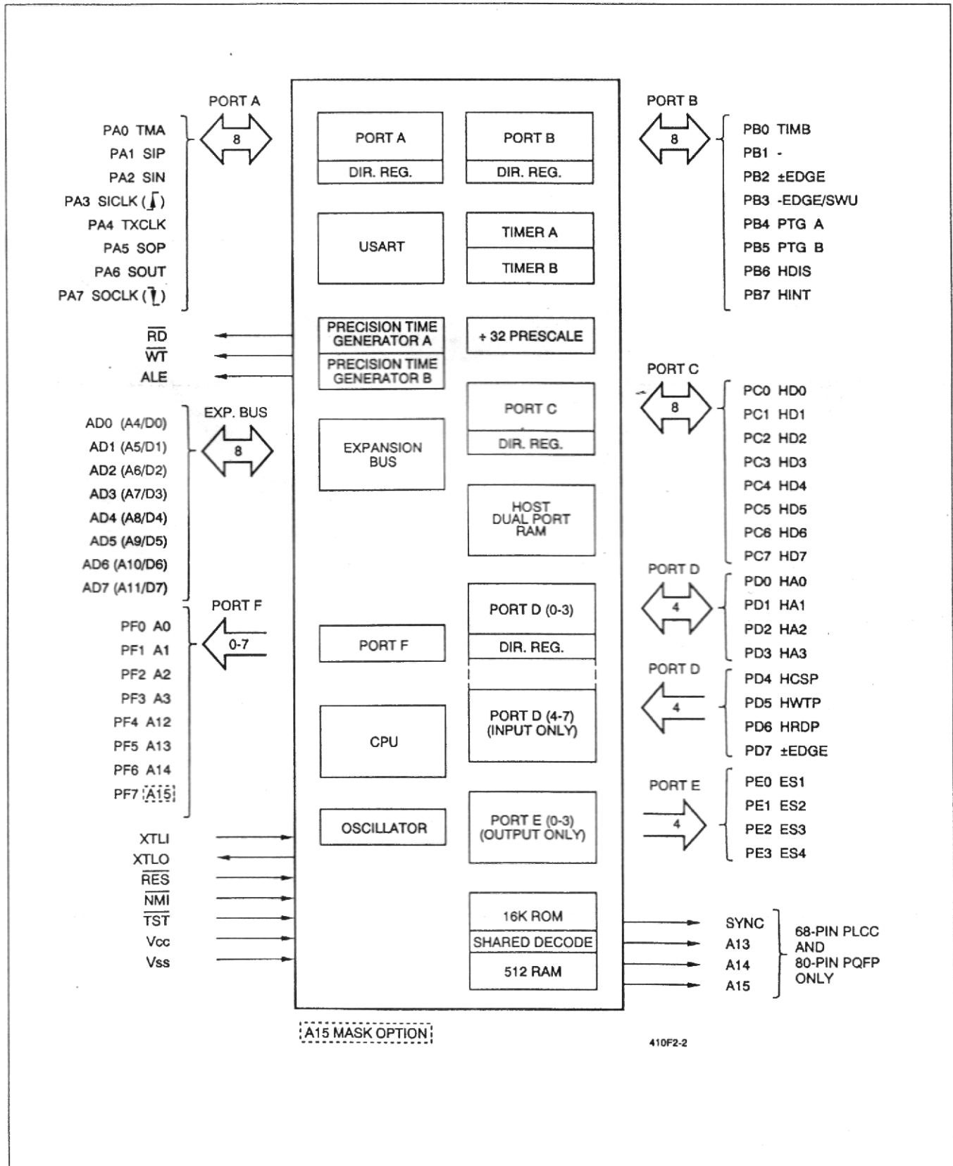
Figure 2-2. R65C19 Internal Functions and I/O Signals
