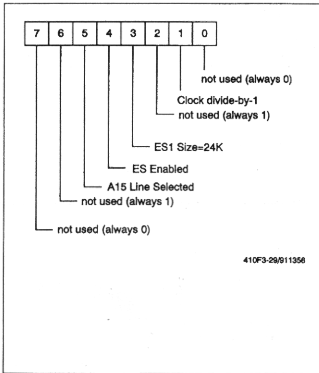
Figure 3-29. Mask Option Register (MOR) - $0008
