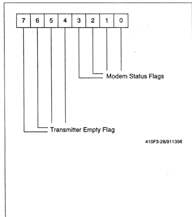
Figure 3-28. Modem Status Register (MSR) - $0031
