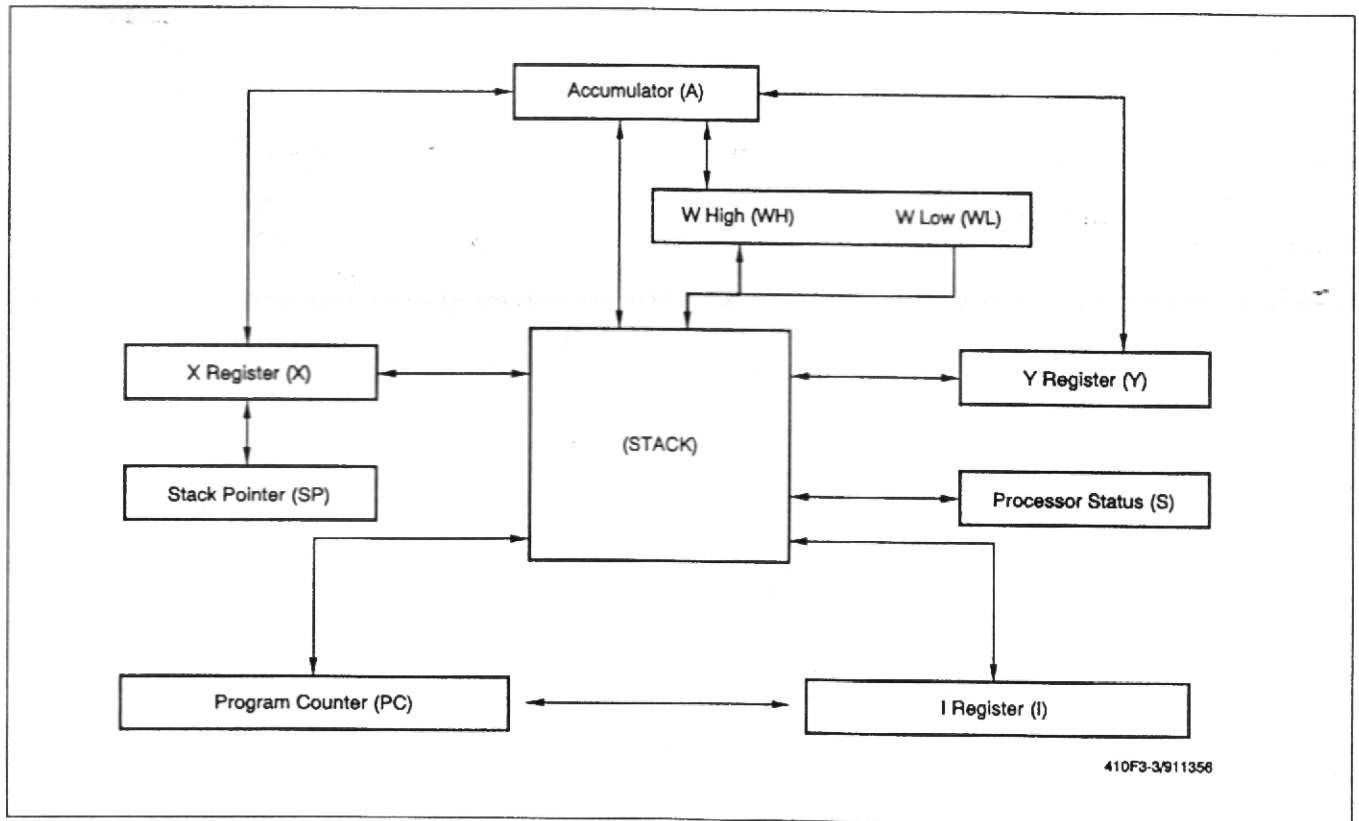
Figure 3-3. CPU Registers and Data Flow
