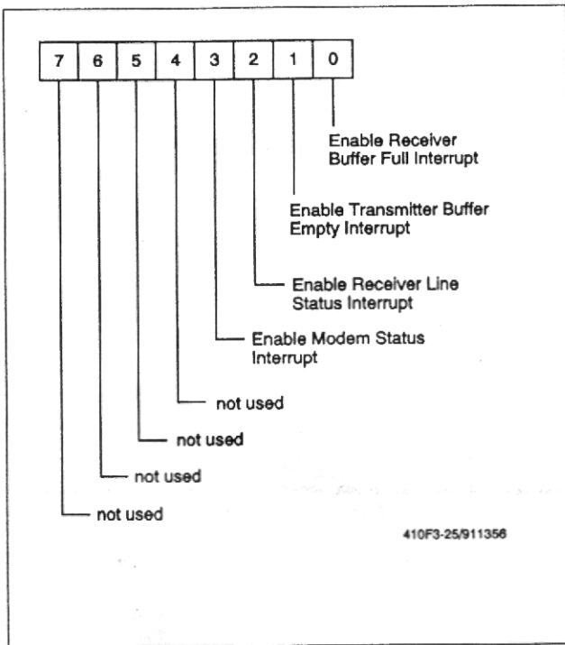
Figure 3-25. Interrupt Enable Register (IER)
