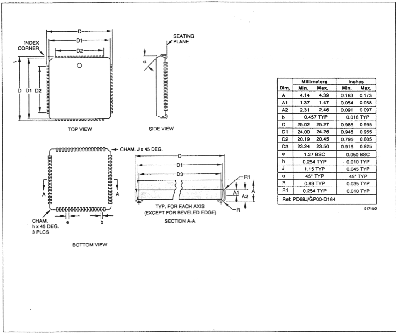
68-Pin PLCC
