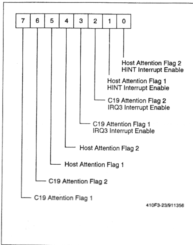
Figure 3-23. Host Handshake Register (HHR) - $002F
