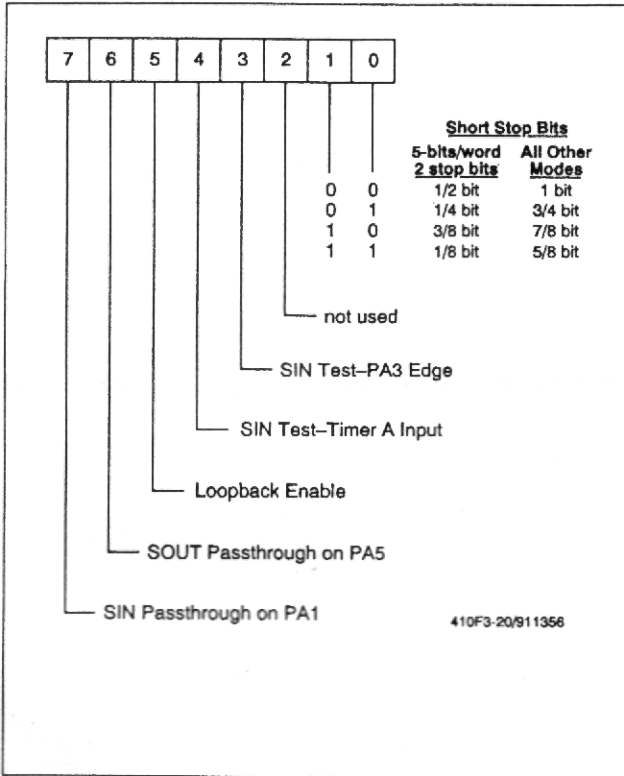
Figure 3-20. Serial Form Register (SFR) - $003D
