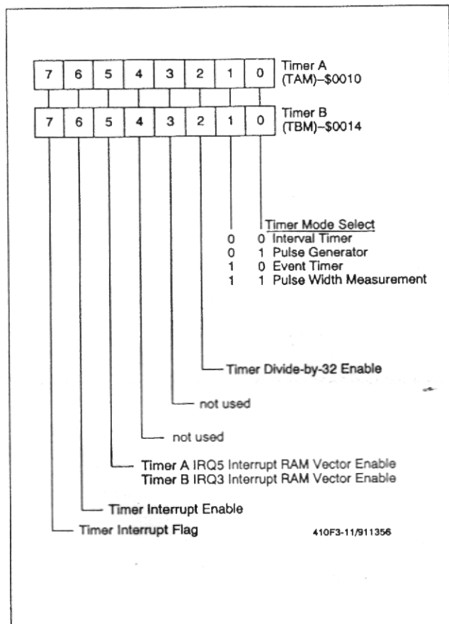
Figure 3-11. Timer A and Timer B Mode Registers
