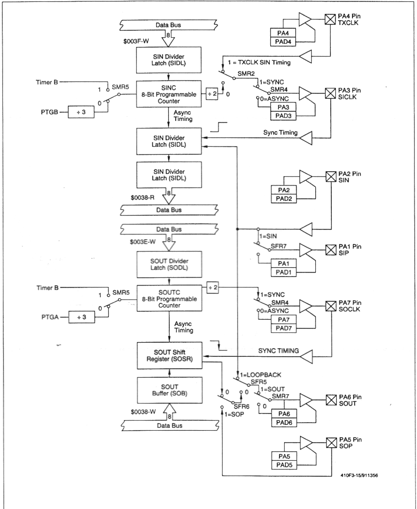
Figure 3-15. USART Block Diagram
