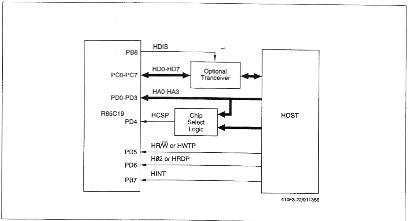
Figure 3-22. Host Bus Interface
