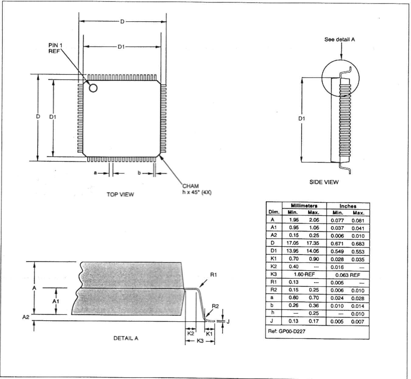
80-Pin PQFP
