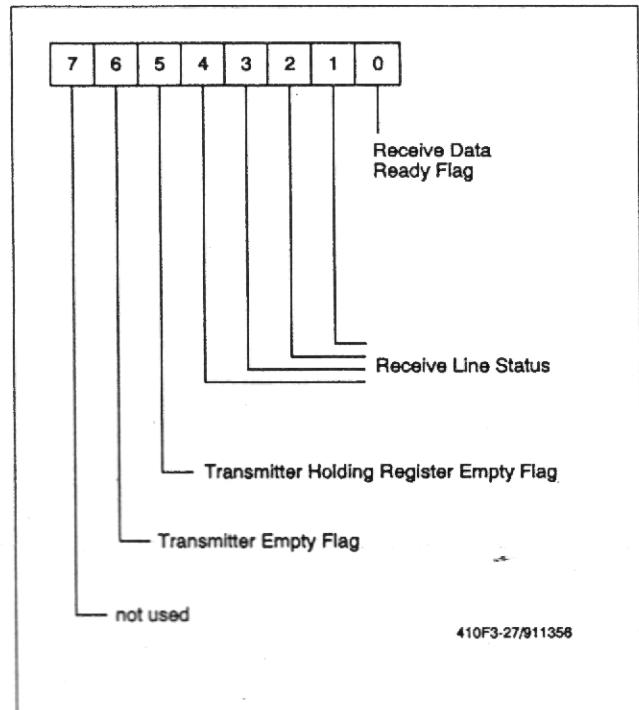
Figure 3-27. Line Status Register (LSR) - $0030
