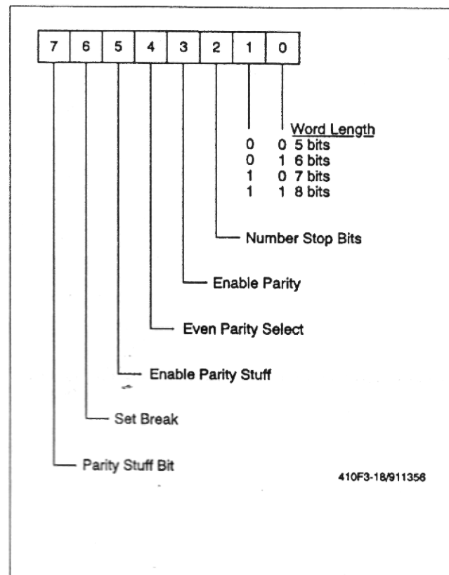
Figure 3-18. Serial Line Register (SLR) - $003B
