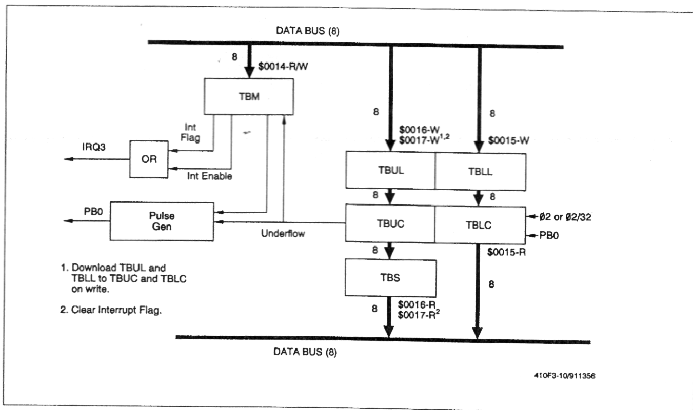
Figure 3-10. Counter/Timer B Block Diagram
