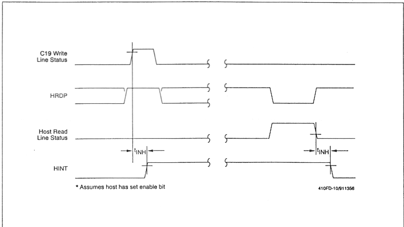
Host Bus Interrupt Timing - 16450 Mode
