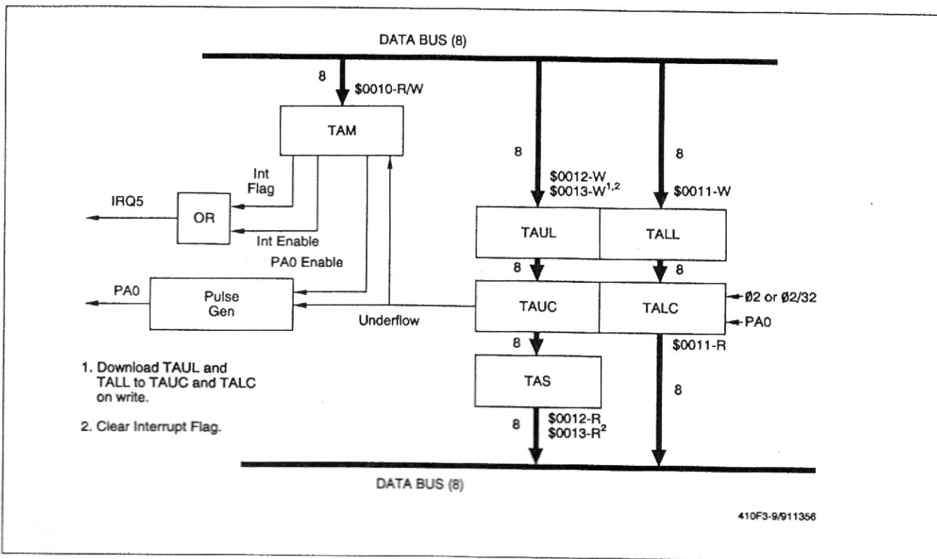
Figure 3-9. Counter/Timer A Block Diagram
