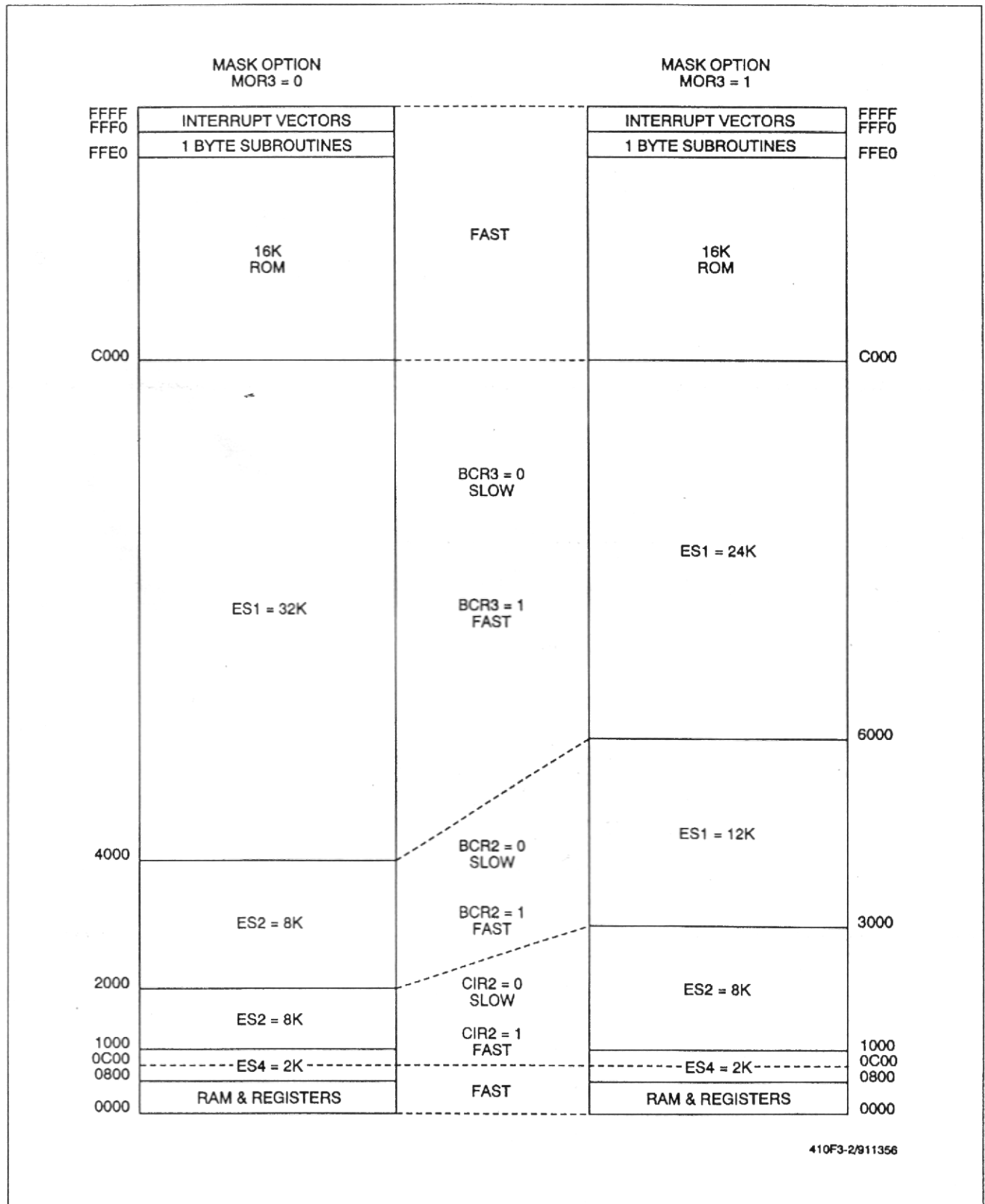
Figure 3-2. Expansion Bus Memory Map
