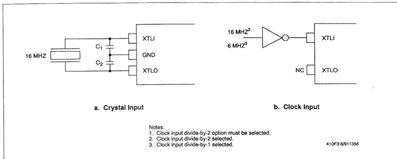
Figure 3-5. Clock Oscillator Input Options
