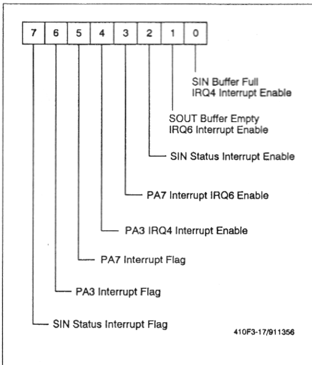
Figure 3-17. Serial Interrupt Register (SIR) - $0039
