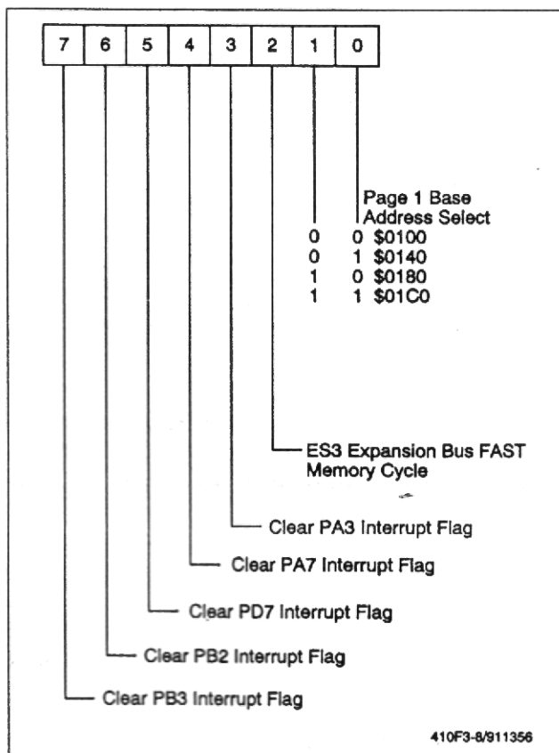
Figure 3-8. Clear Interrupt Register (CIR) - $000B
