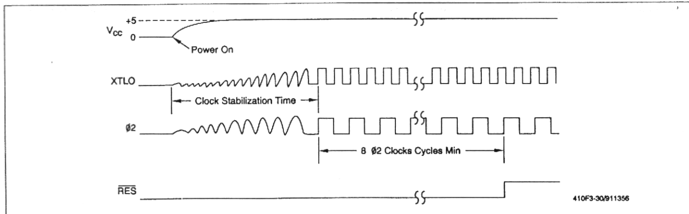
Figure 3-30. Power Turn On Timing Detail
