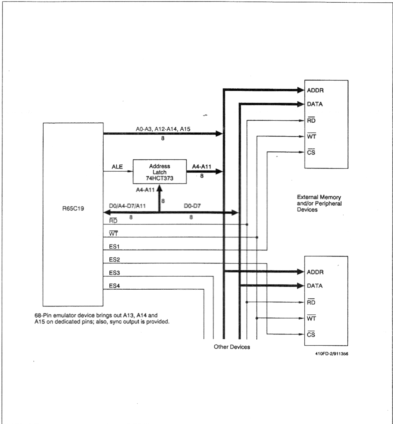
Expansion Bus Interface
