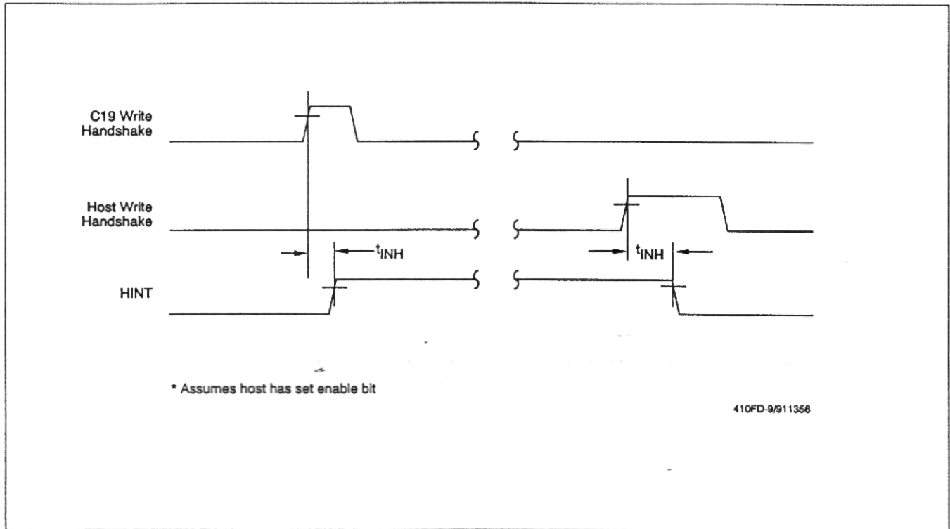
Host Bus Interrupt Timing - GP RAM Mode
