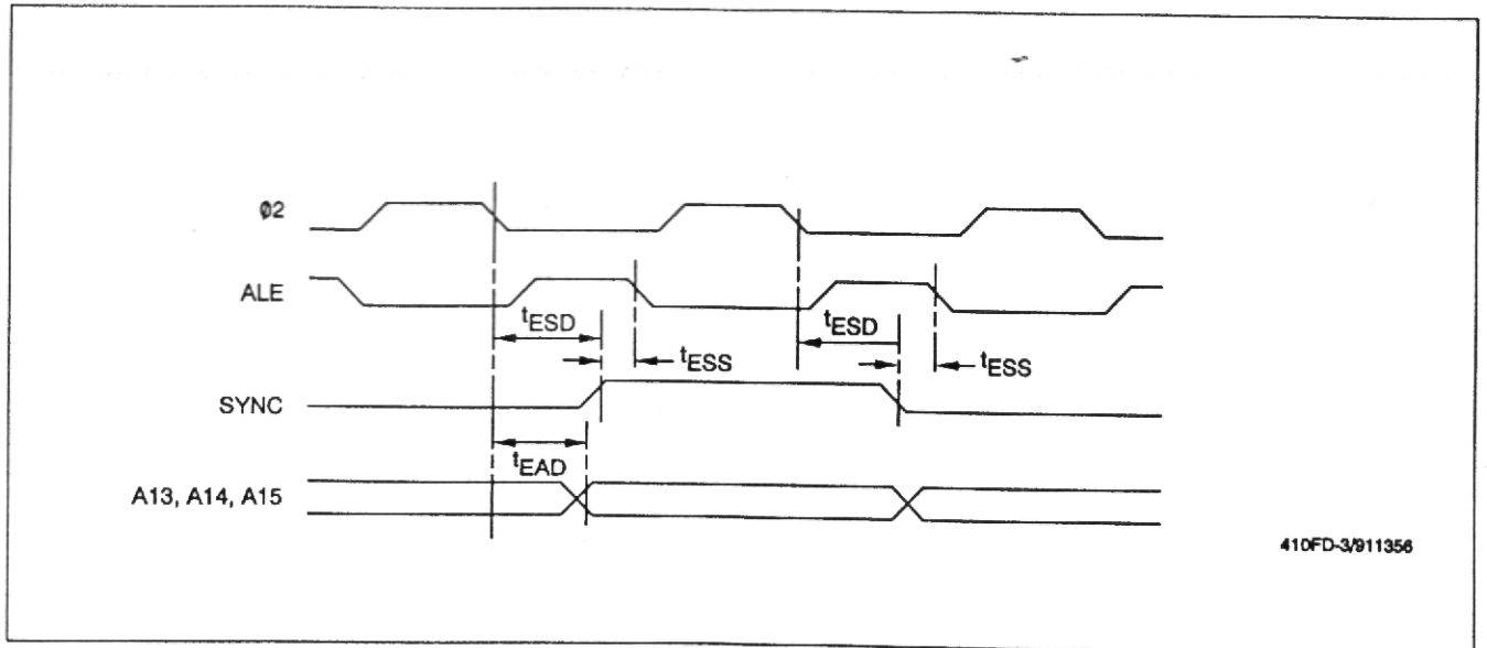
Expansion Bus Waveforms - R65C19 Emulator
