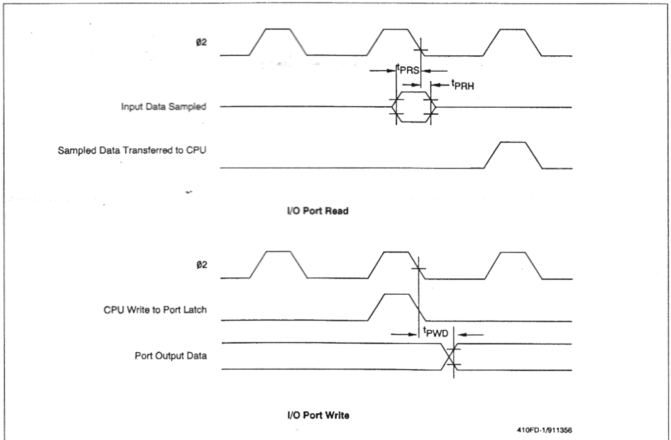
General I/O Waveforms
