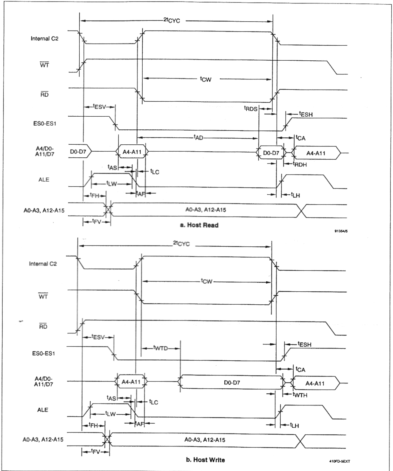
Expansion Bus Timing - Extended
