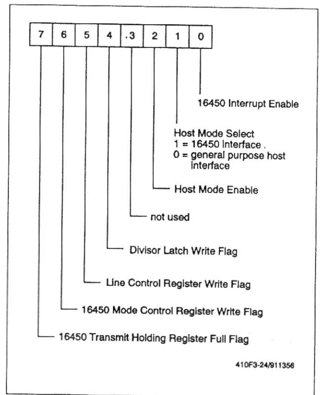
Figure 3-24. Host Control Register (HCR) - $0032
