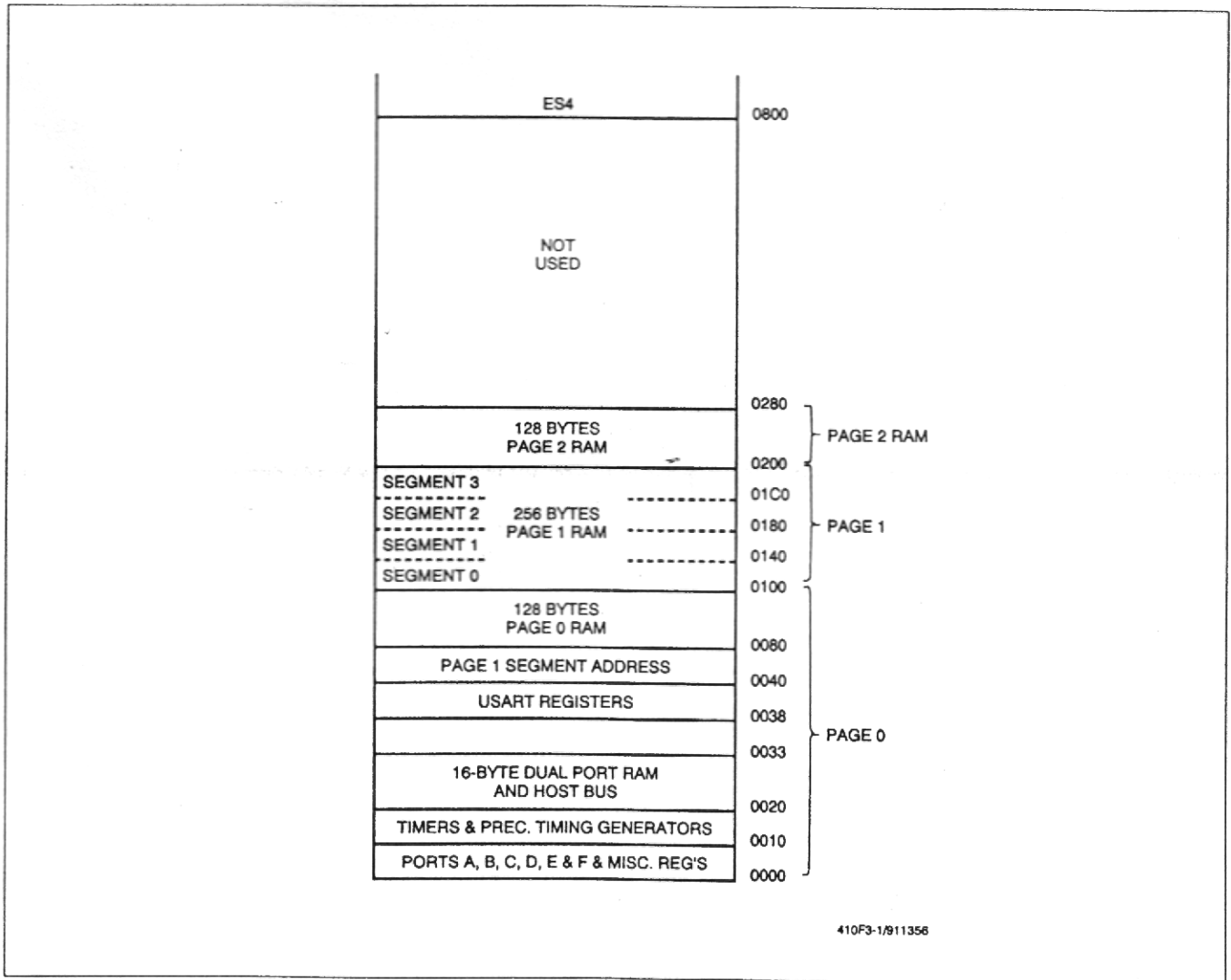
Figure 3-1. RAM Register Memory Map
