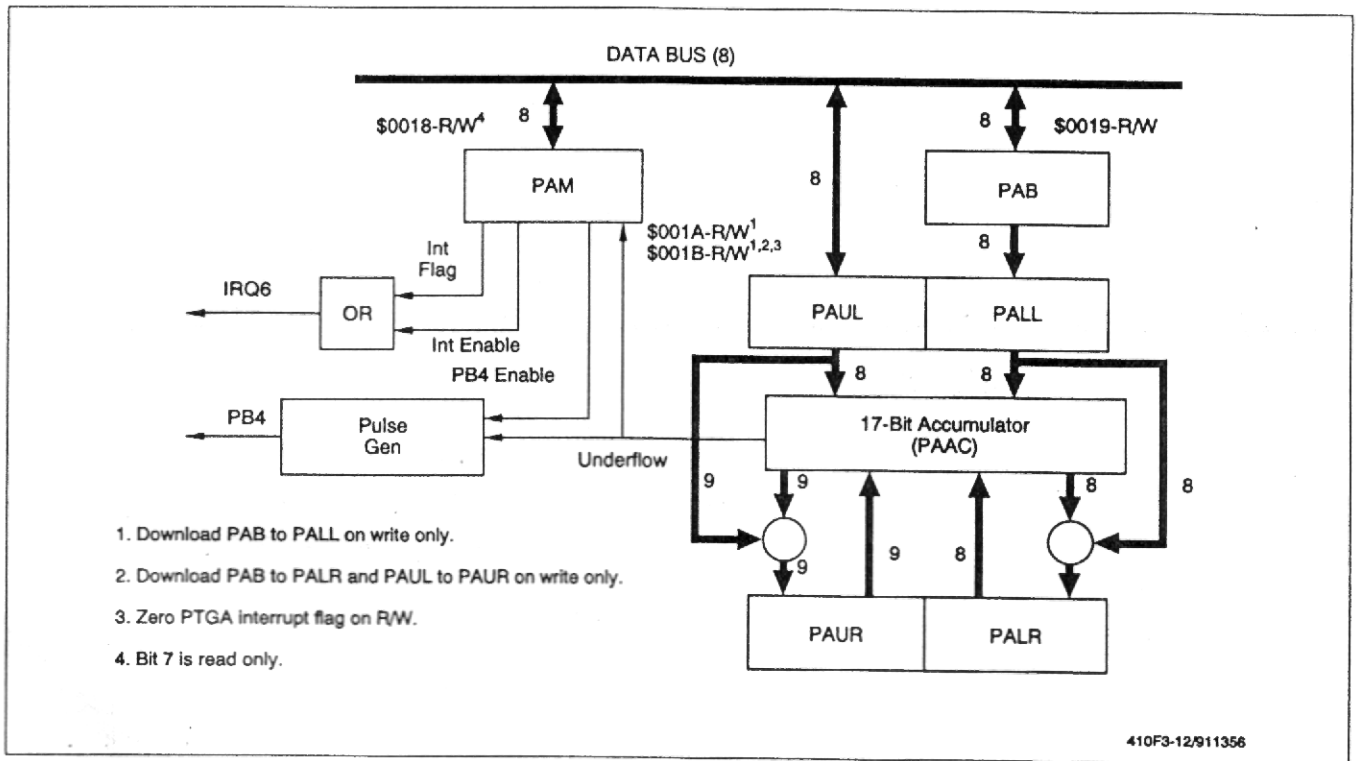
Figure 3-12. Precision Time Generator A
