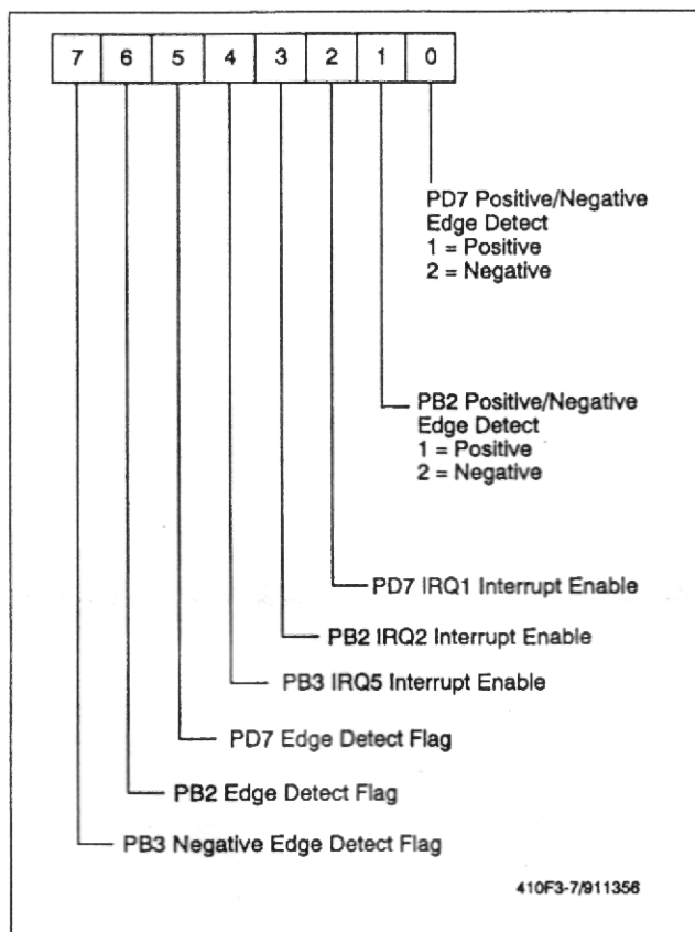
Figure 3-7. External Interrupt Register (EIR) - $000A
