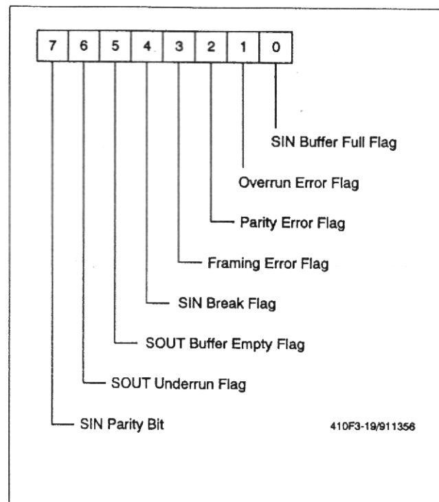
Figure 3-19. Serial Status Register (SSR) - $003C
