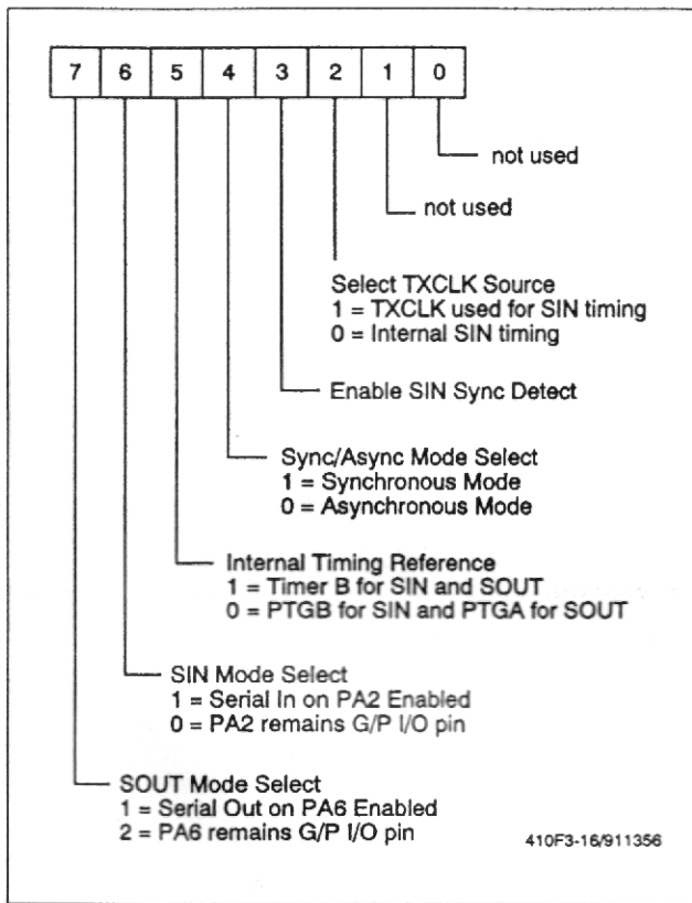
Figure 3-16. Serial Mode Register (SMR) - $003A
