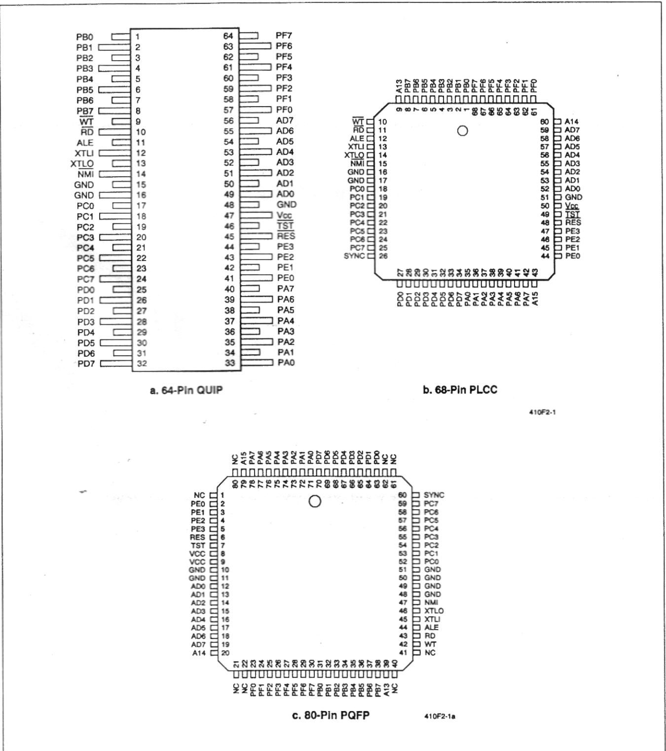
Figure 2-1. R65C19 Pin Assignments
