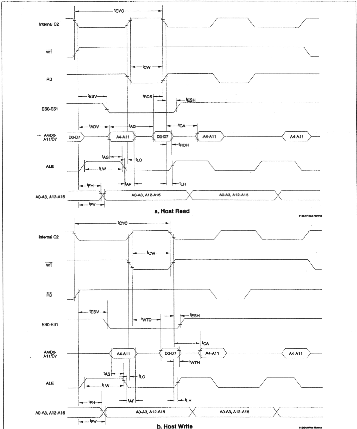
Expansion Bus Timing - Normal
