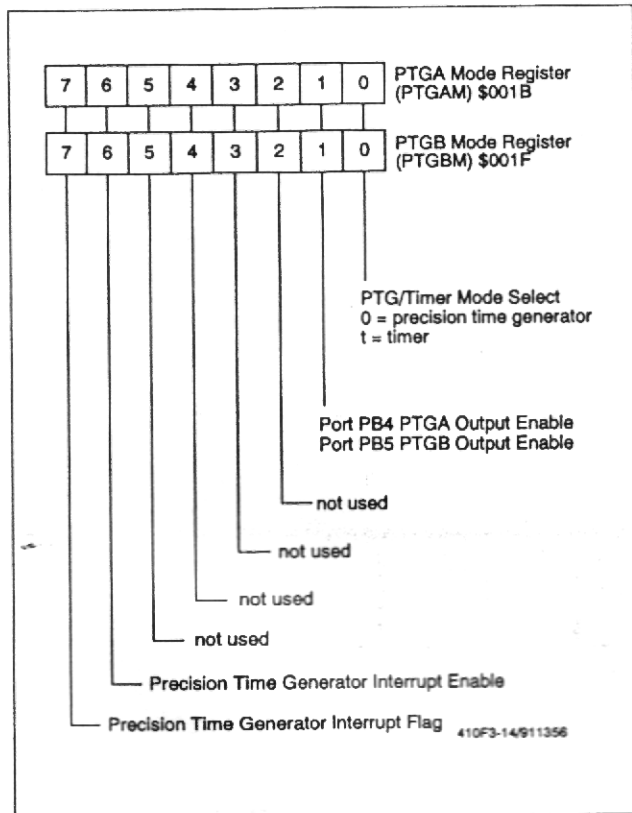
Figure 3-14. PTGA and PTGB Mode Registers
