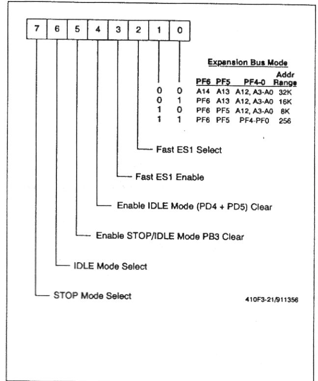
Figure 3-21. Bus Control Register (BCR) - $0009
