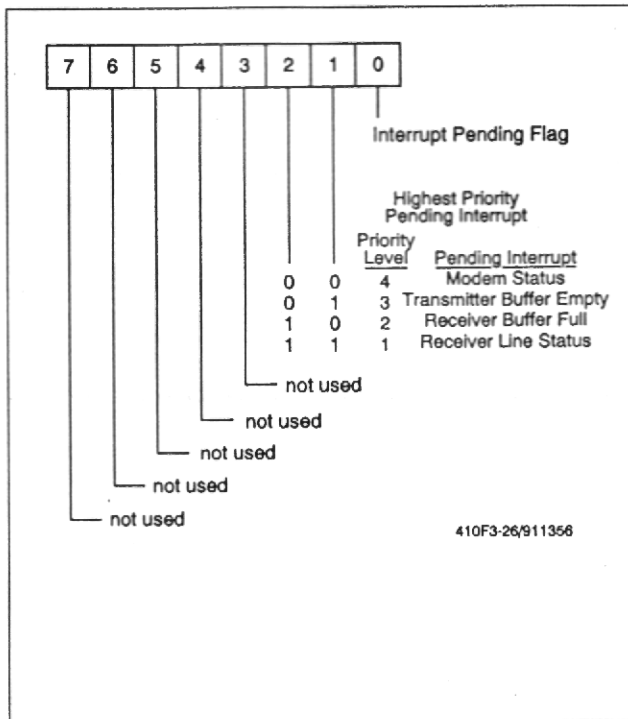
Figure 3-26. Interrupt Identifier Register (SLR)
